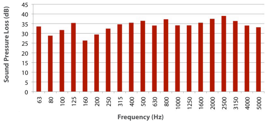
Sound Pressure Loss = dB without enclosure - dB with enclosure
